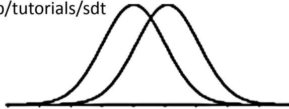
d' = 1 (lots of overlap)
